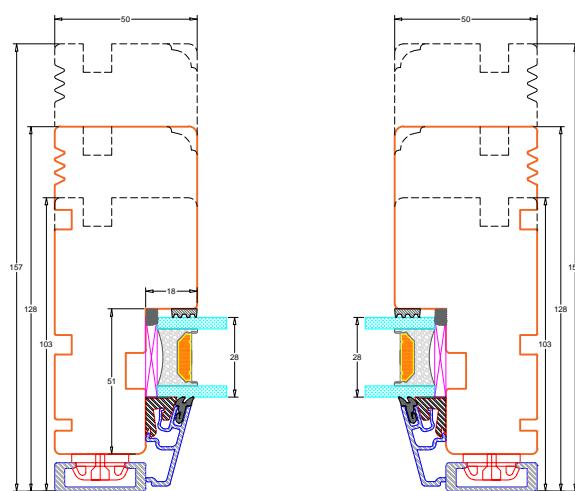
D7: Faste elementer, bund karm
